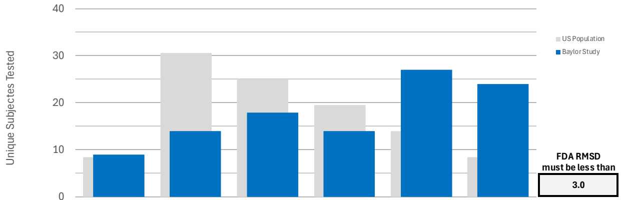
FitzPatrickHistogram
